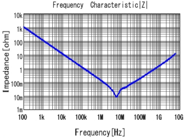
■ GRM188C70J225KE20 |Z| DCOV, 25degC
