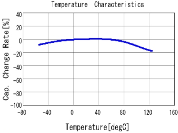
■ GRM188C70J225KE20 C-Temp. capchange, DCO. 0V, ACO. 5V rm
