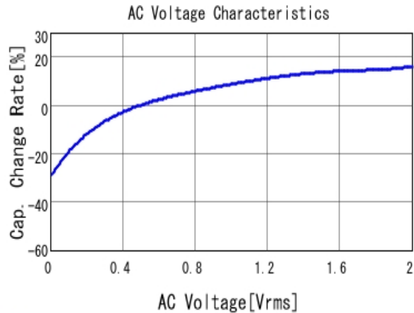
■ GRM188C70J225KE20 C-AC Voltage capchange, DCOV, 25.0d
