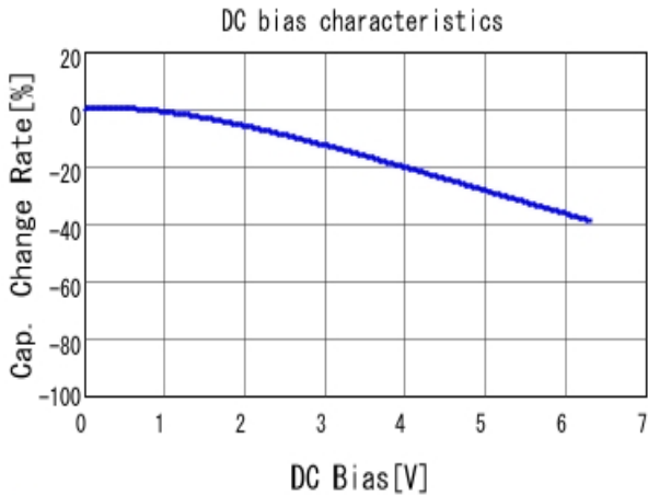
■ GRM188C70J225KE20 C-DC bias capchange, 25.0degC, AC0.
