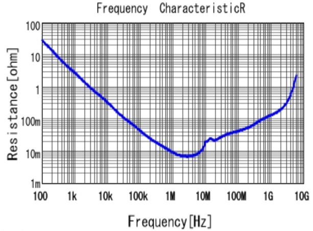
■ GRM188C70J225KE20 R DCOV, 25degC
