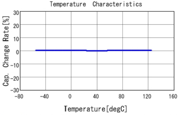
GRM1555C1HR60BA01 C-Temp. capchange, DCOV, AC1Vrms
