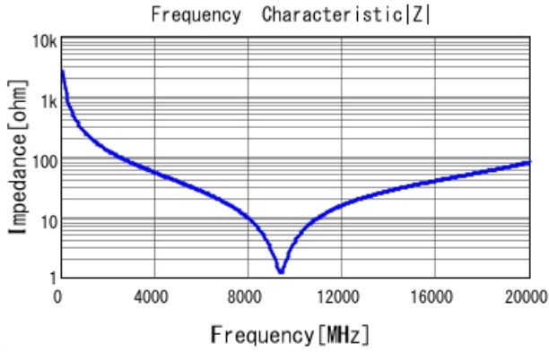
GRM1555C1HR60BA01 |Z| DCOV, 25degC
