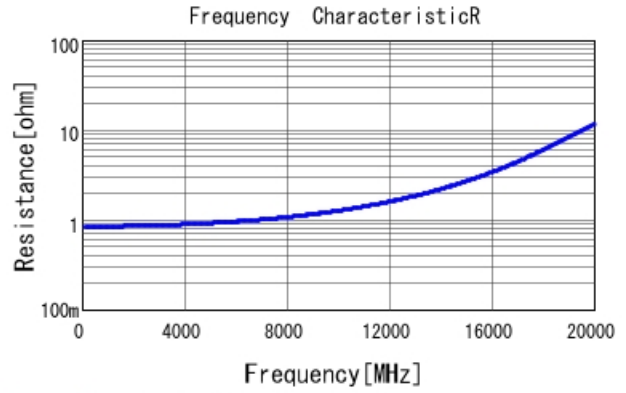
GRM1555C1HR60BA01 R DCOV, 25degC
