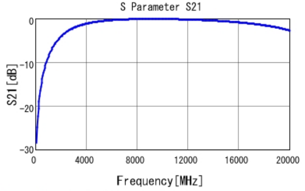
GRM1555C1HR60BA01 S21 DCOV, 25degC
