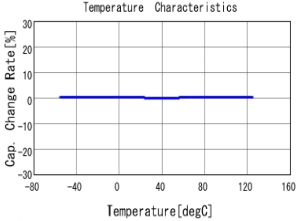
■ GRM1555C2A8R2WA01 C-Temp. capchange, DCOV, AC1Vrms
