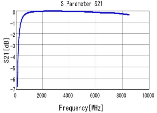
■ GRM1555C2A8R2WA01 S21 DCOV, 25degC
