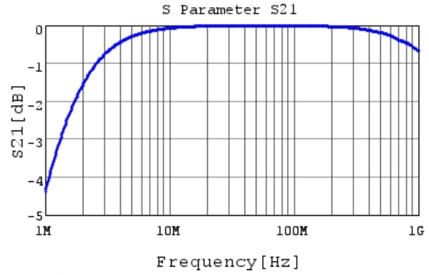
RDE5C1H122J0M1H03A S21 DCOV, 25degC
