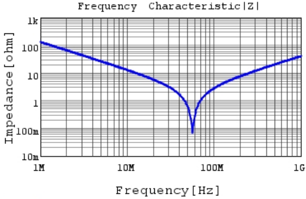
RDE5C1H122J0M1H03A |Z| DCOV, 25degC
