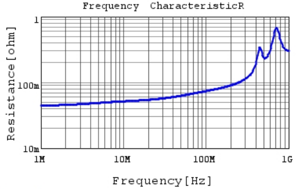
RDE5C1H122J0M1H03A R DCOV, 25degC
