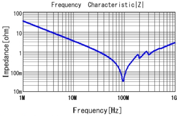
GCM21B5C2E472JX01 |Z| DCOV, 25degC
