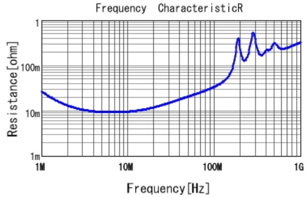
GCM21B5C2E472JX01 R DCOV, 25degC
