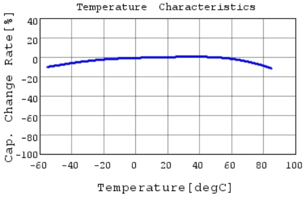
GRT033R61A224KE01 C-Temp. capchange, DC0.0V,
