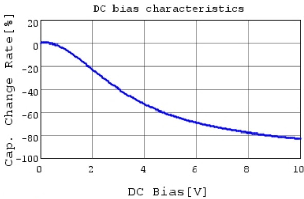
GRT033R61A224KE01 C-DC bias capchange, 25.0c
