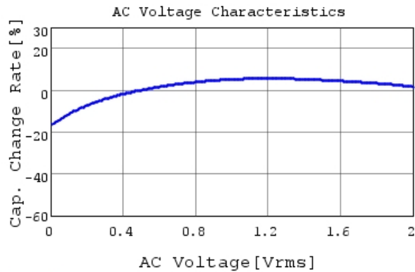
GRT033R61A224KE01 C-AC Voltage capchange, Dc
