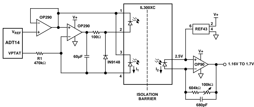
Figure 24. Isolation Amplifier
