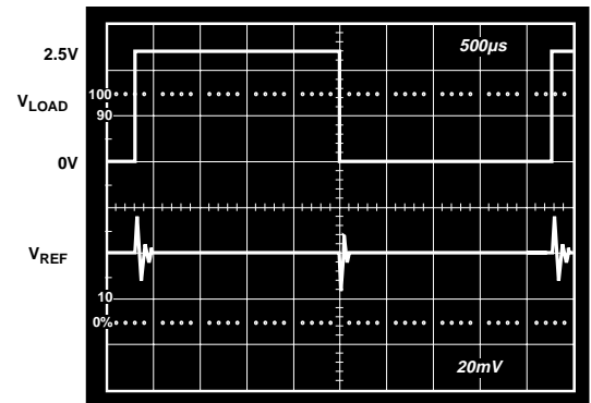
Figure 13. V_{REF} Under Load Switching ( 0\ \mu\text{A} – 500\ \mu\text{A} ), R_{LOAD} = 5\ \text{k}\Omega
