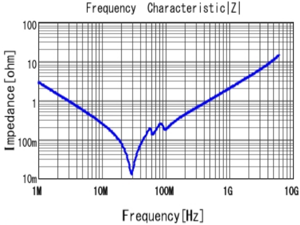
■ GRM2191X1A563JA01 |Z| DCOV, 20degC
