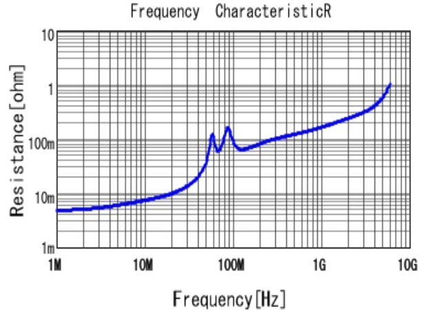
■ GRM2191X1A563JA01 R DCOV, 20degC
