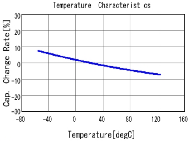
■ GRM2191X1A563JA01 C-Temp. capchange, DCOV, AC1Vrms
