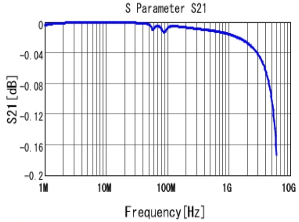
■ GRM2191X1A563JA01 S21 DCOV, 20degC
