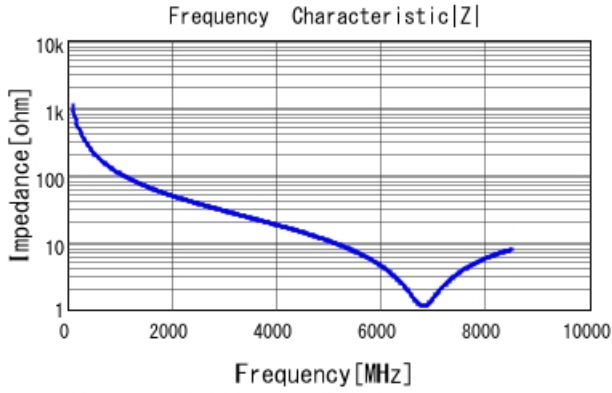
GRM1555C1H1R5BA01 |Z| DCOV, 25degC
