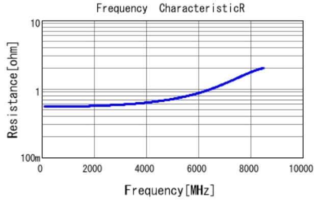
GRM1555C1H1R5BA01 R DCOV, 25degC
