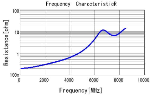
GRM1555C1H7R5WA01 R DCOV, 25degC
