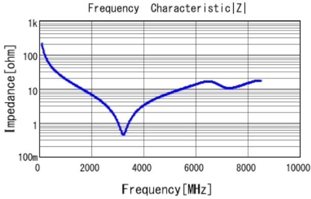
GRM1555C1H7R5WA01 |Z| DCOV, 25degC
