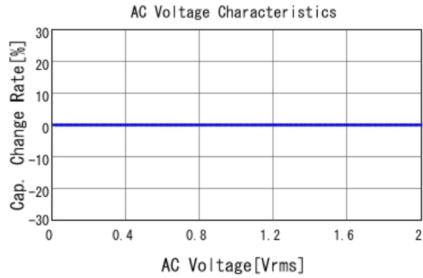
GRM1555C2A7R2BA01 C-AC Voltage capchange, DCOV, 25
