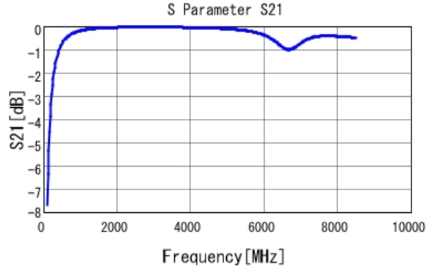
GRM1555C2A7R2BA01 S21 DCOV, 25degC
