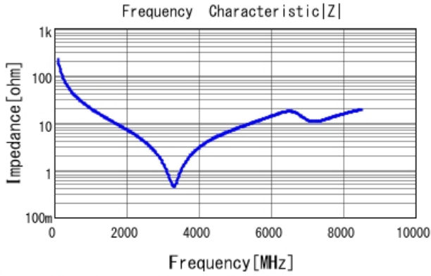
GRM1555C2A7R2BA01 |Z| DCOV, 25degC
