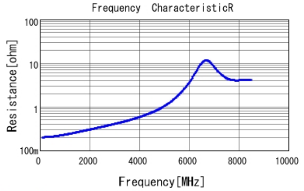
GRM1555C2A7R2BA01 R DCOV, 25degC
