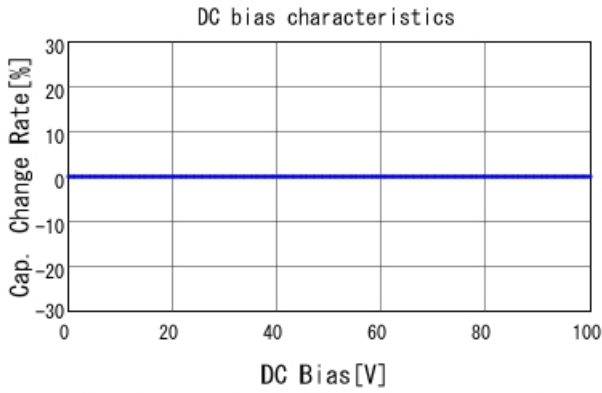
GRM1555C2A7R2BA01 C-DC bias capchange, 25.0degC, A
