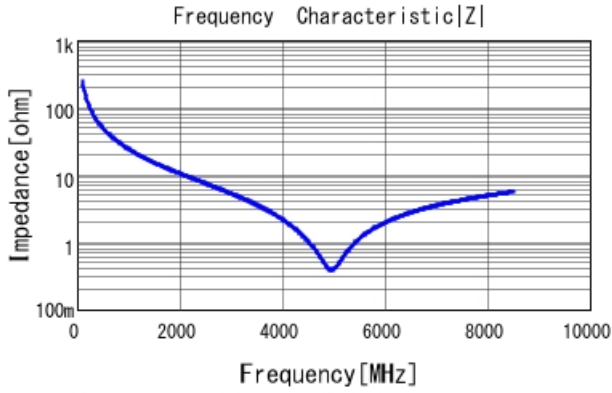
GRM0225C1E6R3CA03 |Z| DCOV, 25degC
