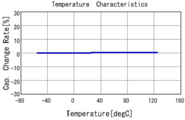
GRM0225C1E6R3CA03 C-Temp. capchange, DC0V, AC1Vrms
