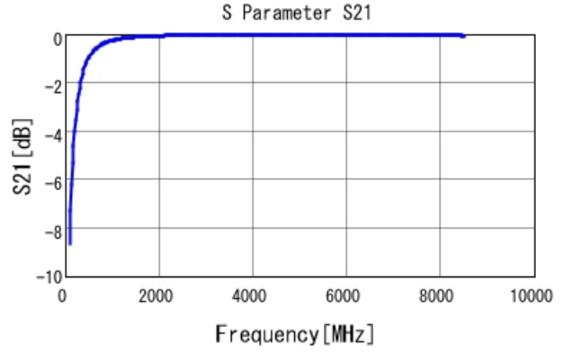
GRM0225C1E6R3CA03 S21 DC0V, 25degC
