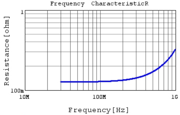
RDE5C2A151J0M1H03A R DCOV, 25degC
