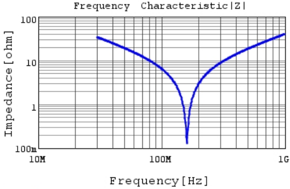
RDE5C2A151J0M1H03A |Z| DCOV, 25degC
