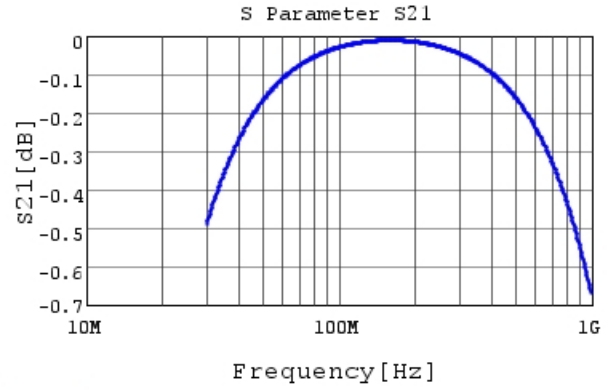
RDE5C2A151J0M1H03A S21 DCOV, 25degC
