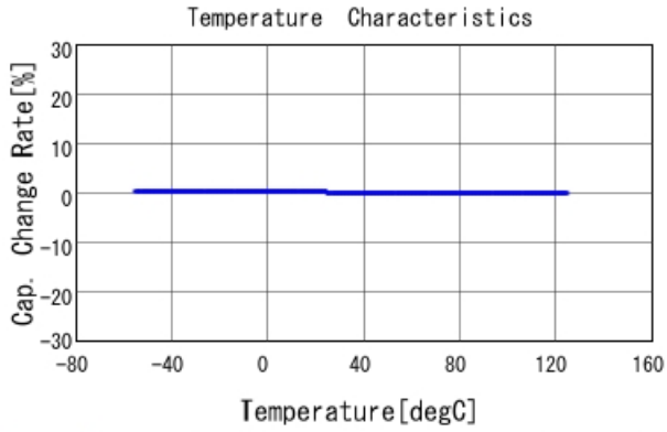
GRM0335C1H3R9BA01 C-Temp. capchange, DCOV, AC1Vrms
