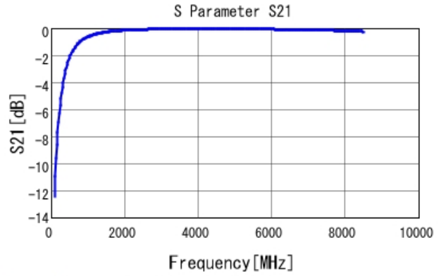
GRM0335C1H3R9BA01 S21 DCOV, 25degC
