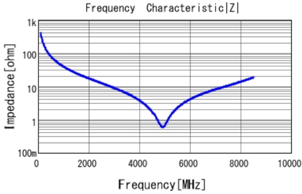
GRM0335C1H3R9BA01 |Z| DCOV, 25degC
