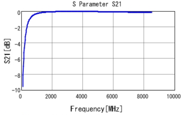
GRM0335C1H5R6CA01 S21 DC0V, 25degC
