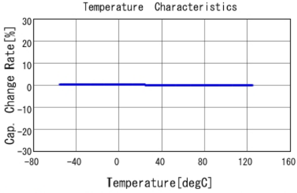
GRM0335C1H5R6CA01 C-Temp. capchange, DC0V, AC1Vrms
