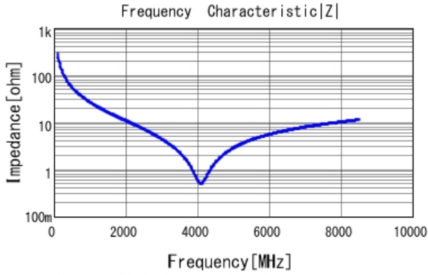
GRM0335C1H5R6CA01 |Z| DCOV, 25degC
