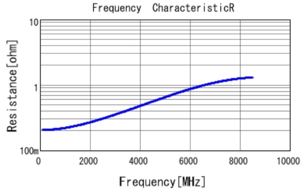
GRM0335C1H5R6CA01 R DCOV, 25degC
