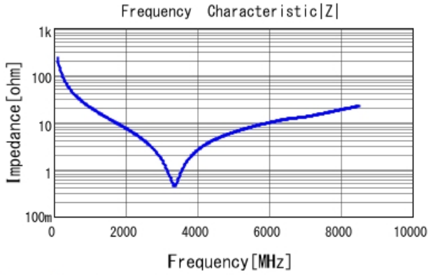
GRM1555C2A6R9CA01 |Z| DCOV, 25degC
