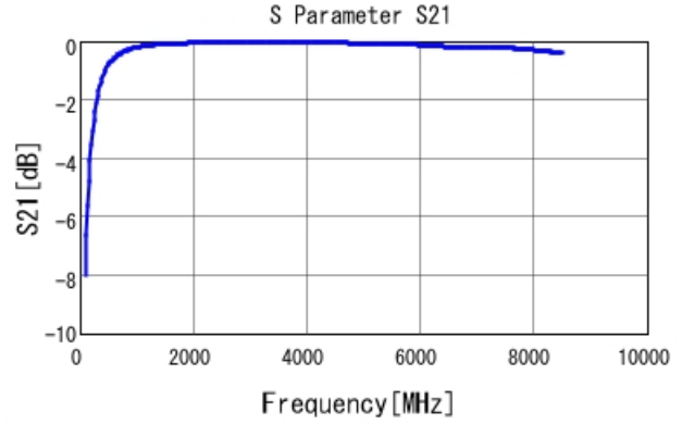
GRM1555C2A6R9CA01 S21 DCOV, 25degC
