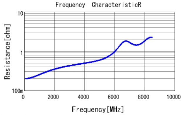
GRM1555C2A6R9CA01 R DCOV, 25degC
