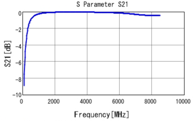
GRM1555C1H6R1BA01 S21 DCOV, 25degC
