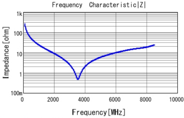
GRM1555C1H6R1BA01 |Z| DCOV, 25degC
