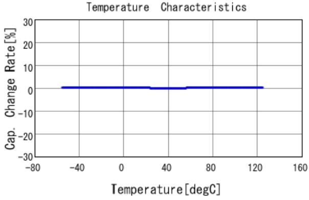
GRM1555C1H6R1BA01 C-Temp. capchange, DCOV, AC1Vrms
