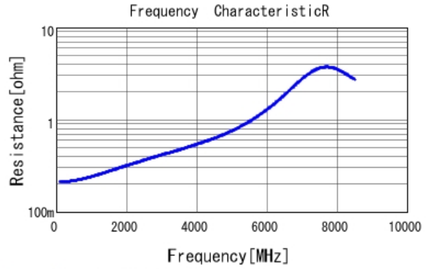
GRM1555C1H6R1BA01 R DCOV, 25degC
