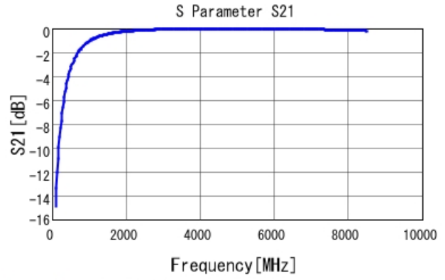
GJM1555C1H2R9CB01 S21 DC0V, 25degC
