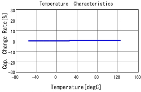
GJM1555C1H2R9CB01 C-Temp. capchange, DC0V, AC1Vrms
