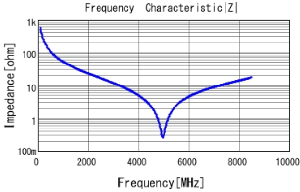
GJM1555C1H2R9CB01 |Z| DCOV, 25degC
