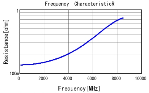
GJM1555C1H2R9CB01 R DCOV, 25degC
