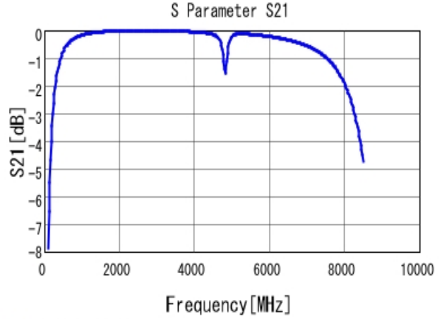
■ GQM1885C1H7R0DB01 S21 DCOV, 25degC
