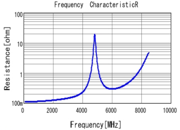
■ GQM1885C1H7R0DB01 R DCOV, 25degC
