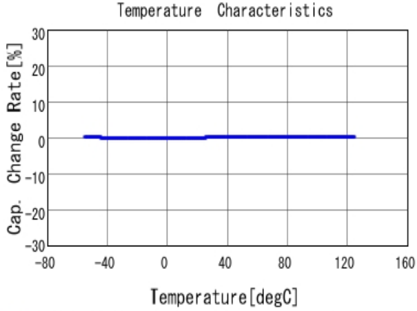
■ GQM1885C1H7R0DB01 C-Temp. capchange, DCOV, AC1Vrms
