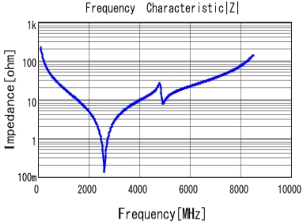
■ GQM1885C1H7R0DB01 |Z| DCOV, 25degC
