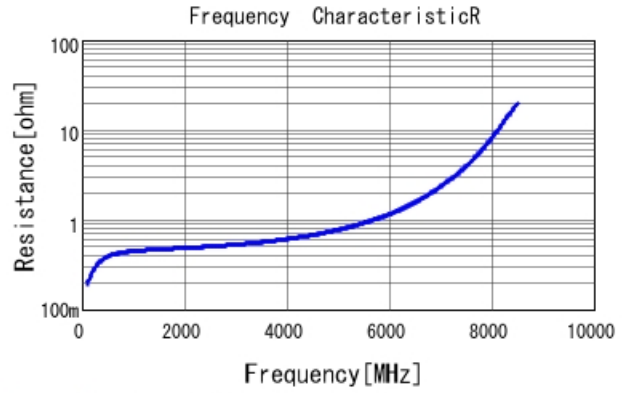
GRM1885C2A2R0BA01 R DCOV, 25degC
