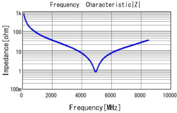
GRM1885C2A2R0BA01 |Z| DCOV, 25degC
