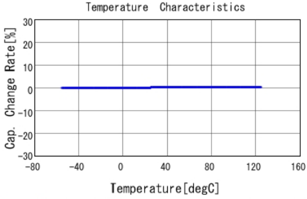
GRM1885C2A2R0BA01 C-Temp. capchange, DCOV, AC1Vrms
