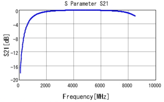
GRM1885C2A2R0BA01 S21 DCOV, 25degC
