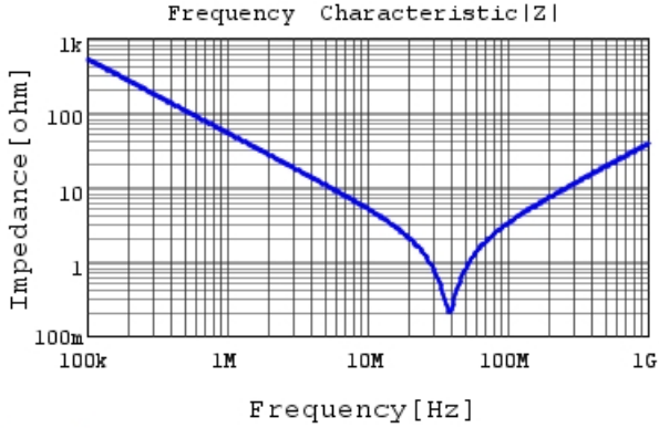
RDER72J332K2K1H03B |Z| DCOV,25degC
