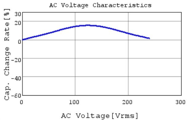
RDER72J332K2K1H03B C-AC Voltage capchange, I
