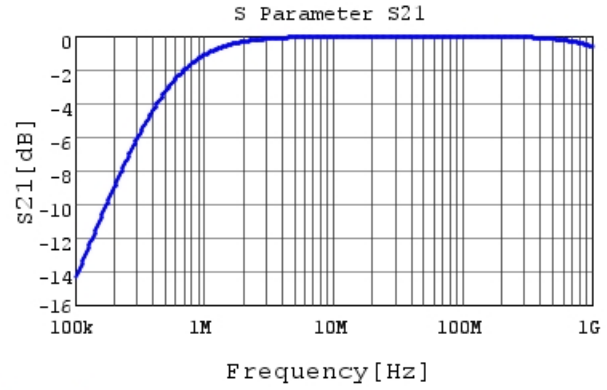
RDER72J332K2K1H03B S21 DCOV, 25degC
