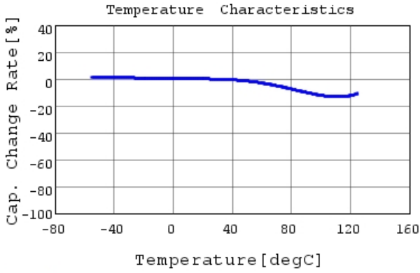
RDER72J332K2K1H03B C-Temp. capchange, DCOV,
