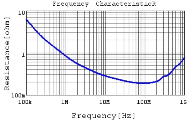
RDER72J332K2K1H03B R DCOV,25degC
