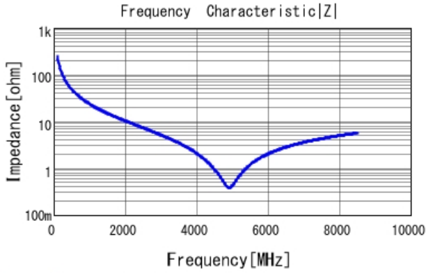
GRM0225C1E6R4CA03 |Z| DCOV, 25degC
