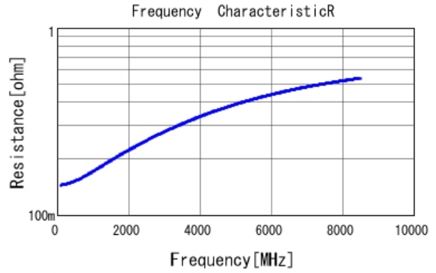
GRM0225C1E6R4CA03 R DCOV, 25degC
