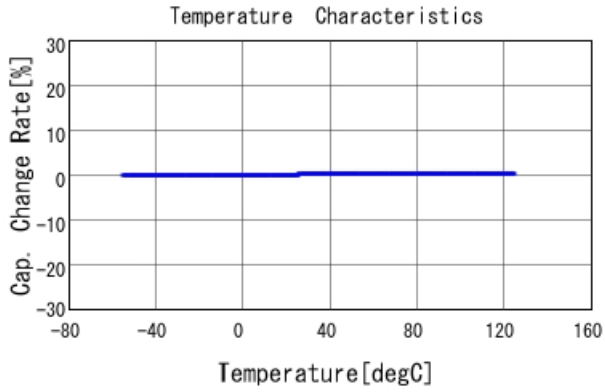
GRM0225C1E6R4CA03 C-Temp. capchange, DC0V, AC1Vrms
