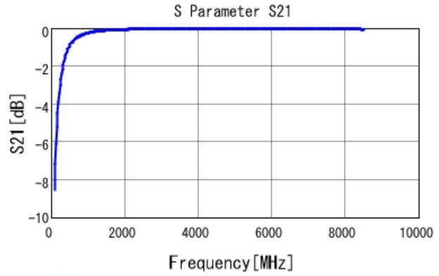
GRM0225C1E6R4CA03 S21 DC0V, 25degC
