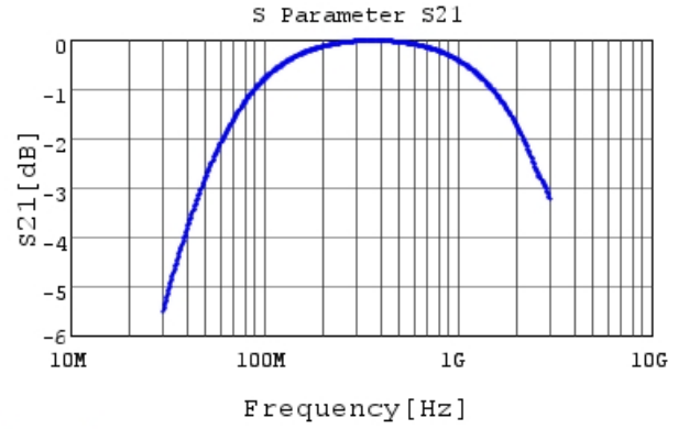
RDE5C1H330J0P1H03B S21 DCOV, 25degC
