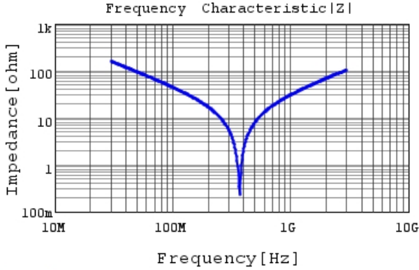
RDE5C1H330J0P1H03B |Z| DC0V, 25degC
