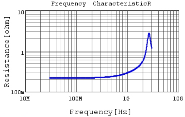
RDE5C1H330J0P1H03B R DC0V, 25degC
