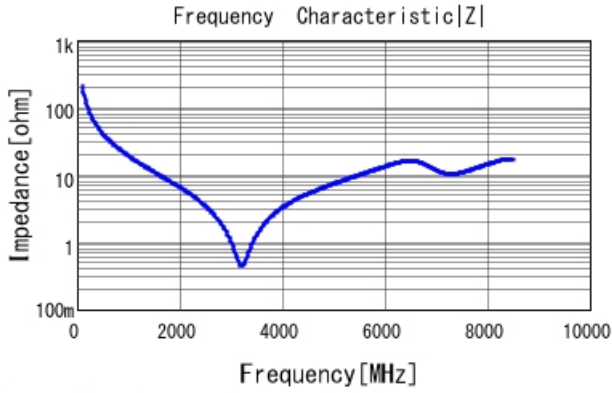
GRM1555C2A7R6BA01 |Z| DCOV, 25degC
