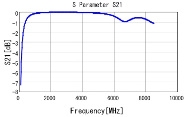
GRM1555C2A7R6BA01 S21 DCOV, 25degC
