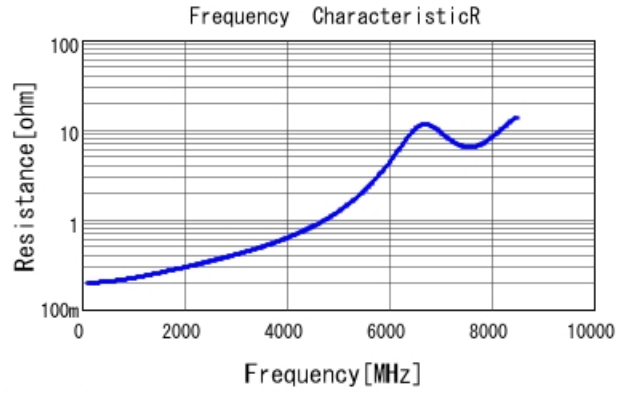
GRM1555C2A7R6BA01 R DCOV, 25degC
