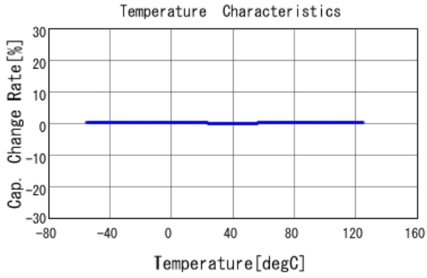
GRM1555C2A7R6BA01 C-Temp. capchange, DCOV, AC1Vrms
