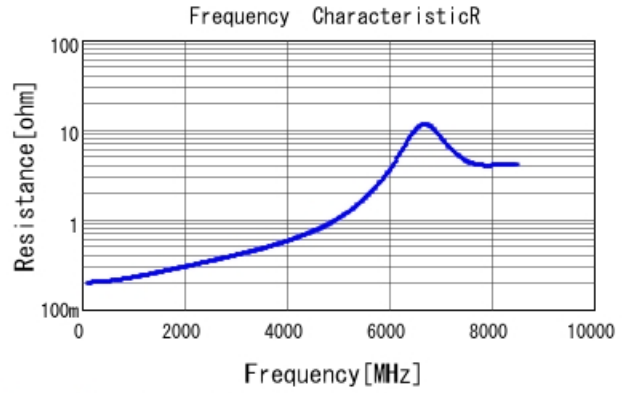
GRM1555C2A7R1BA01 R DCOV, 25degC
