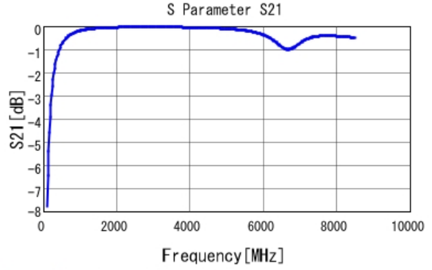
GRM1555C2A7R1BA01 S21 DCOV, 25degC
