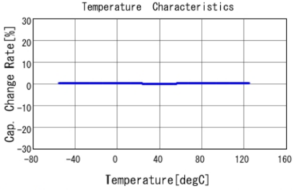
GRM1555C2A7R1BA01 C-Temp. capchange, DCOV, AC1Vrms
