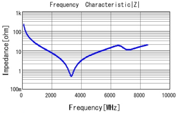
GRM1555C2A7R1BA01 |Z| DCOV, 25degC
