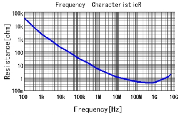
■ GRT033R71E471KE01 R DC0V, 25degC
