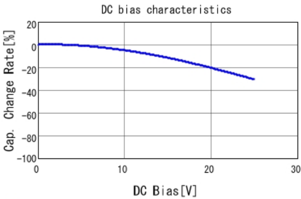
■ GRT033R71E471KE01 C-DC bias capchange, 25.0degC, AC1.
