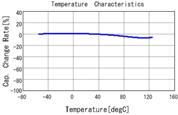
■ GRT033R71E471KE01 C-Temp. capchange, DCO. 0V, AC1. 0Vrm
