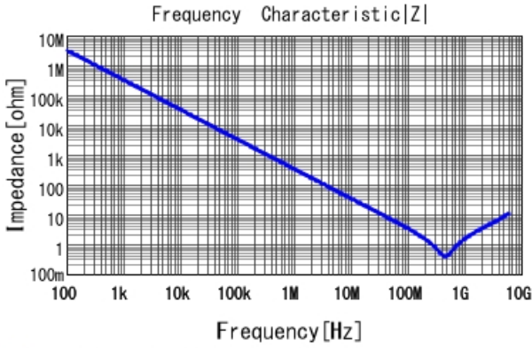
■ GRT033R71E471KE01 |Z| DC0V, 25degC
