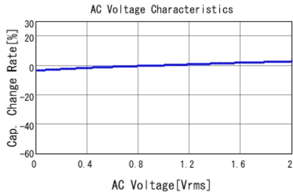
■ GRT033R71E471KE01 C-AC Voltage capchange, DC0V, 25.0d
