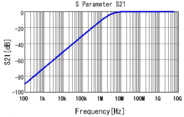
■ GRT033R71E471KE01 S21 DCOV, 25degC
