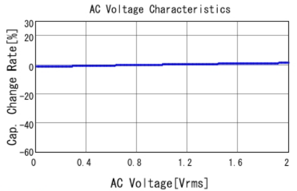
GCJ216R72A272KA01 C-AC Voltage capchange, DCOV, 25
