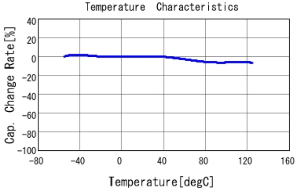
GCJ216R72A272KA01 C-Temp. capchange, DC0.0V, AC1.C
