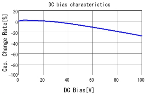
GCJ216R72A272KA01 C-DC bias capchange, 25.0degC, A
