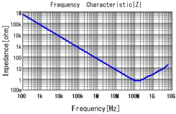
GCJ216R72A272KA01 |Z| DCOV, 25degC
