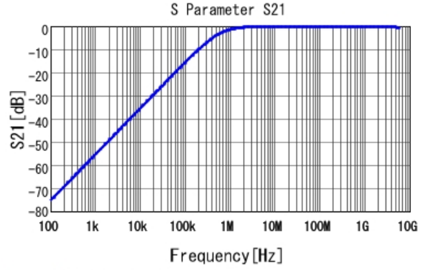
GCJ216R72A272KA01 S21 DC0V, 25degC
