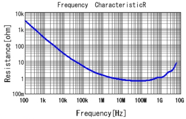
GCJ216R72A272KA01 R DCOV, 25degC
