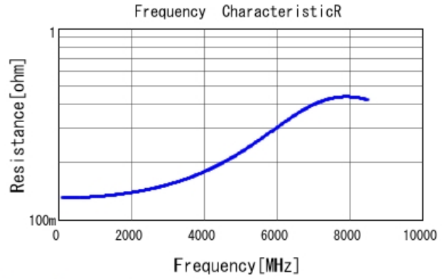
GJM0335C1E3R4BB01 R DCOV, 25degC
