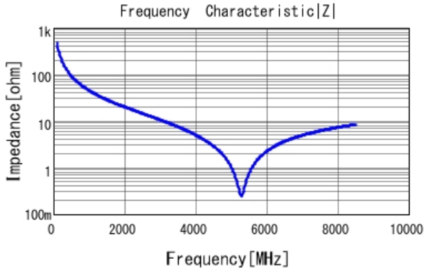
GJM0335C1E3R4BB01 |Z| DCOV, 25degC
