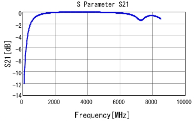
GRM1885C2A4R1BA01 S21 DC0V, 25degC
