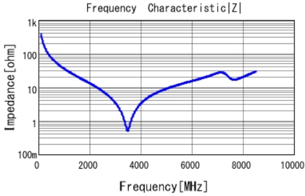
GRM1885C2A4R1BA01 |Z| DCOV, 25degC
