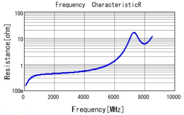
GRM1885C2A4R1BA01 R DCOV, 25degC
