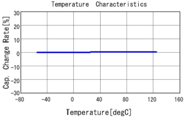
GRM1885C2A4R1BA01 C-Temp. capchange, DC0V, AC1Vrms
