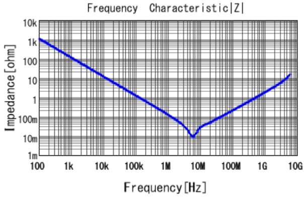
GCH188C71A225KE01 |Z| DC0V, 25degC
