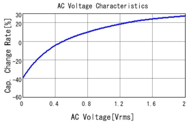
GCH188C71A225KE01 C-AC Voltage capchange, DC0V, 25.0d
