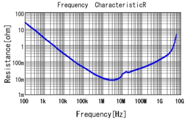
GCH188C71A225KE01 R DC0V, 25degC
