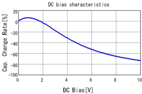
GCH188C71A225KE01 C-DC bias capchange, 25.0degC, AC0.
