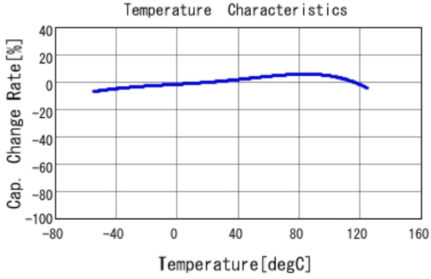
GCH188C71A225KE01 C-Temp. capchange, DCO. 0V, ACO. 5Vrm
