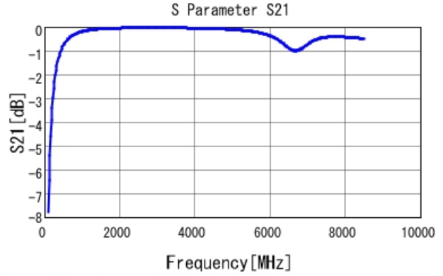
GRM1555C2A7R1WA01 S21 DCOV, 25degC
