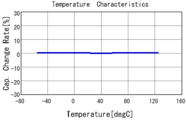
GRM1555C2A7R1WA01 C-Temp. capchange, DCOV, AC1Vrms
