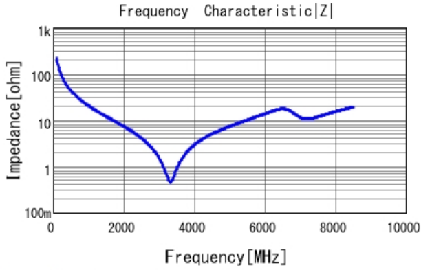
GRM1555C2A7R1WA01 |Z| DCOV, 25degC
