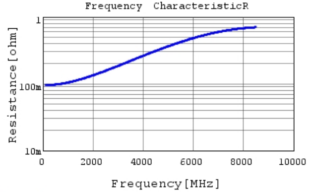
GJM0335C1E9R0DB01 R DC0V, 25degC
