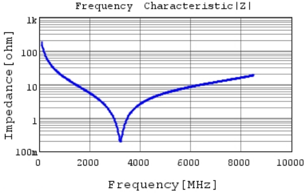
GJM0335C1E9R0DB01 |Z| DC0V, 25degC
