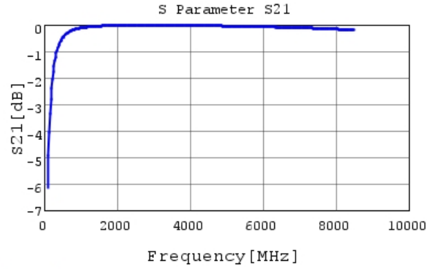
GJM0335C1E9R0DB01 S21 DCOV, 25degC
