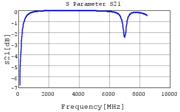
GQM1555C2D8R2CB01 S21 DCOV, 25degC
