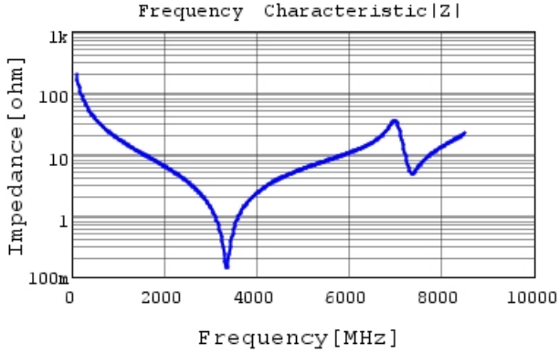
GQM1555C2D8R2CB01 |Z| DC0V, 25degC
