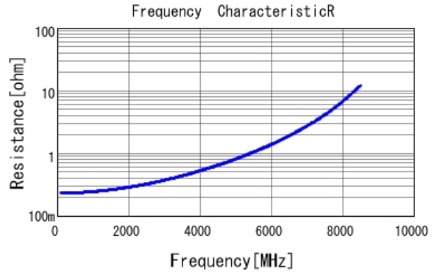
GRM1555C1H3R8CA01 R DCOV, 25degC
