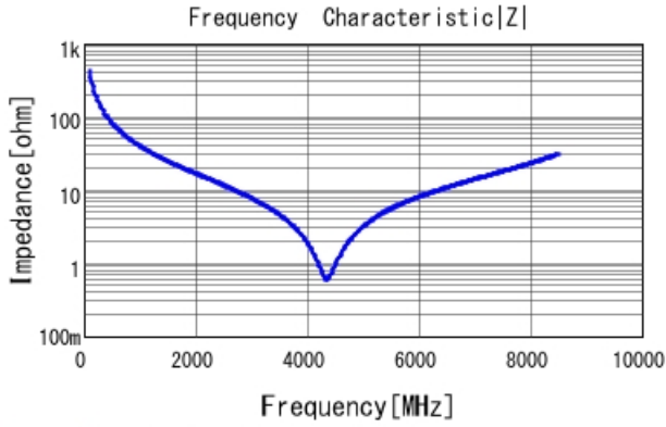
GRM1555C1H3R8CA01 |Z| DCOV, 25degC
