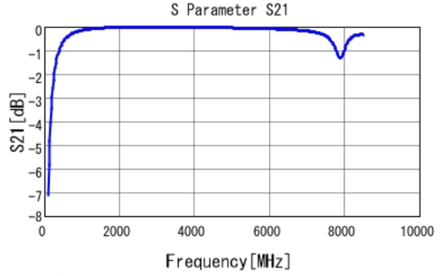
GJM1555C1H7R8CB01 S21 DC0V, 25degC
