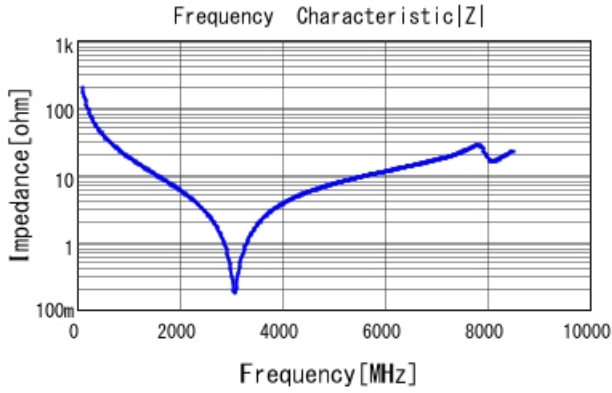
GJM1555C1H7R8CB01 |Z| DCOV, 25degC
