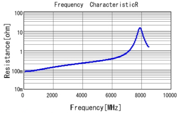
GJM1555C1H7R8CB01 R DCOV, 25degC
