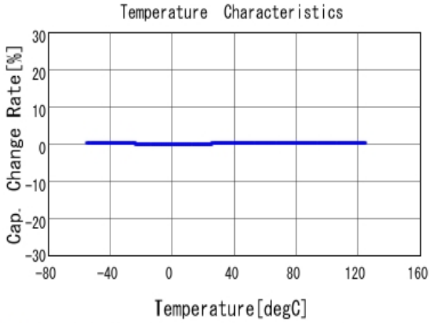
GQM2195C2E1R6CB12 C-Temp. capchange, DCOV, AC1Vrms
