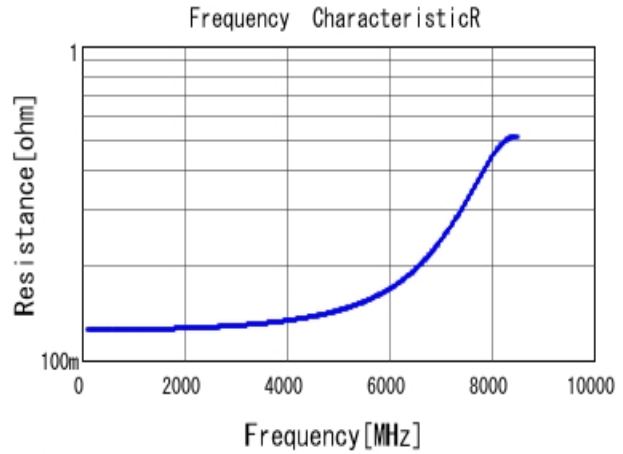
■ GQM2195C2E1R6CB12 R DCOV, 25degC
