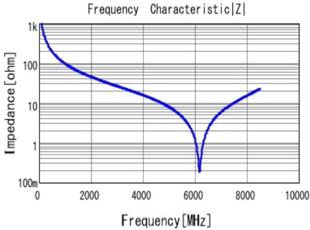
■ GQM2195C2E1R6CB12 |Z| DCOV, 25degC
