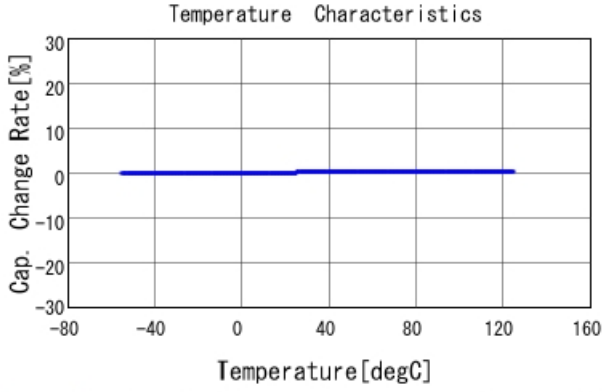
GRM1885C2A3R2WA01 C-Temp. capchange, DCOV, AC1Vrms
