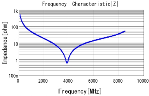
GRM1885C2A3R2WA01 |Z| DCOV, 25degC
