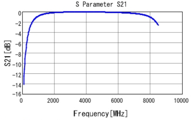
GRM1885C2A3R2WA01 S21 DCOV, 25degC
