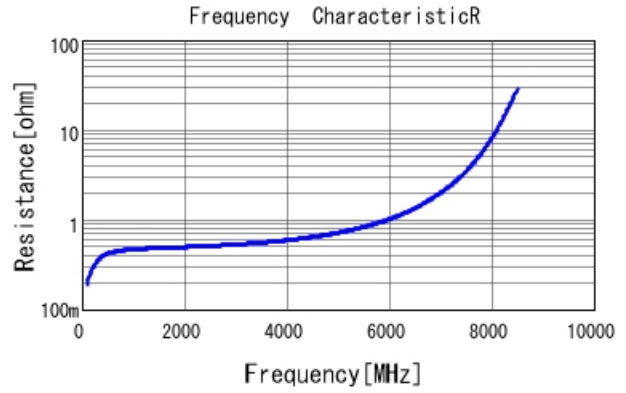
GRM1885C2A3R2WA01 R DCOV, 25degC
