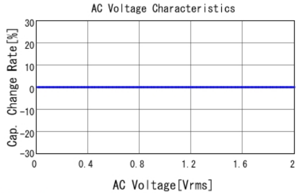
GRM1885C2A3R2WA01 C-AC Voltage capchange, DCOV, 25
