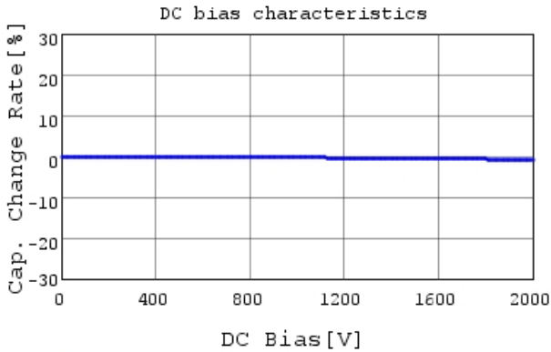
GRM31A7U3D150JW31 C-DC bias capchange, 25.0c
