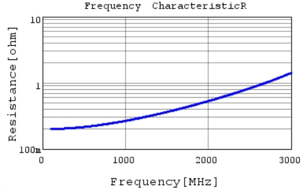
GRM31A7U3D150JW31 R DC0V, 25degC
