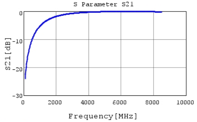
GCM1885C2A1R0CA16 S21 DCOV, 25degC
