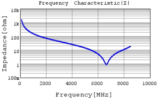
GCM1885C2A1R0CA16 |Z| DCOV, 25degC
