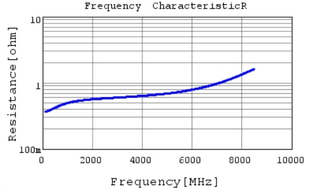
GCM1885C2A1R0CA16 R DCOV, 25degC
