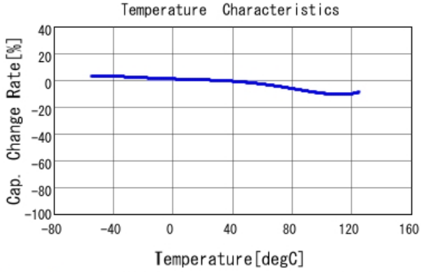
GCM188R71E473KA37 C-Temp. capchange, DC0.0V, AC1.C
