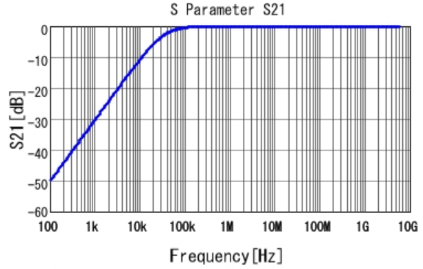
GCM188R71E473KA37 S21 DC0V, 25degC
