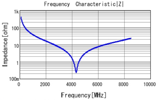
GJM1555C1H4R0BB01 |Z| DCOV, 25degC
