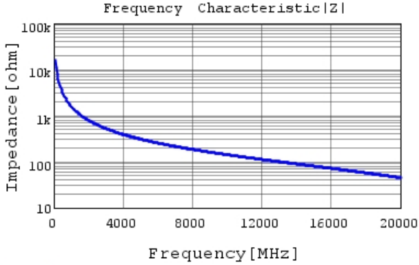
GRM0335C1ER10WA01 |Z| DCOV, 25degC
