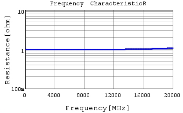
GRM0335C1ER10WA01 R DCOV, 25degC
