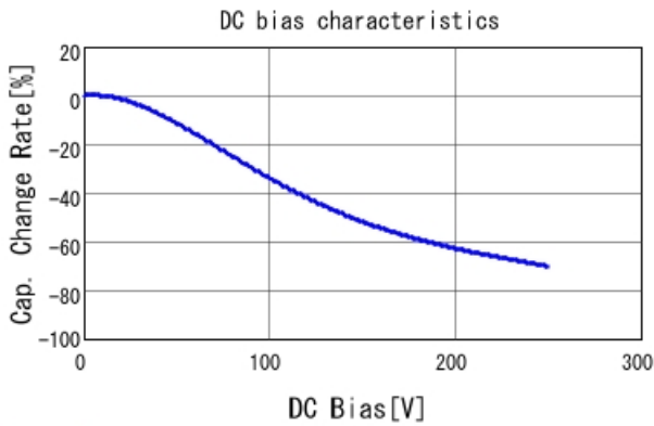
GRJ21AR72E472KWJ1 C-DC bias capchange, 25.0degC, A
