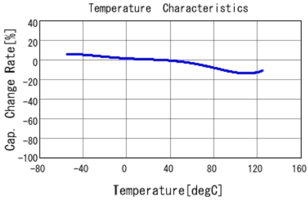
GRJ21AR72E472KWJ1 C-Temp. capchange, DCOV, AC1Vrms
