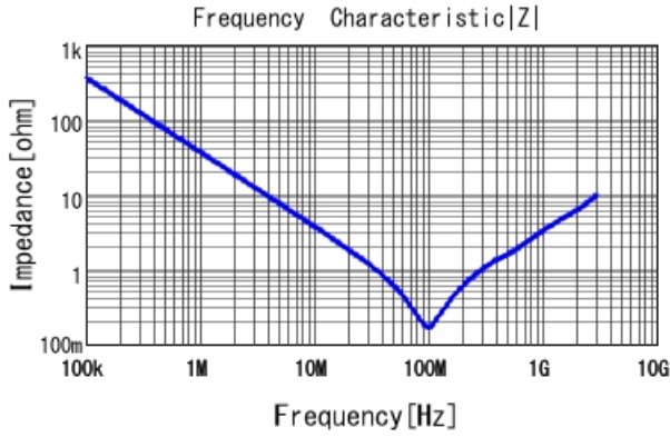
GRJ21AR72E472KWJ1 |Z| DCOV, 25degC
