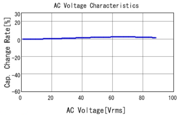
GRJ21AR72E472KWJ1 C-AC Voltage capchange, DCOV, 25
