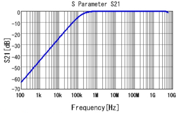
GRM188R71E103KA01 S21 DC0V, 25degC
