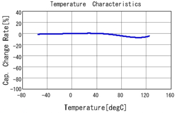
GRM188R71E103KA01 C-Temp. capchange, DC0.0V, AC1.C
