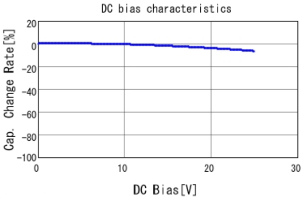
GRM188R71E103KA01 C-DC bias capchange, 25.0degC, A
