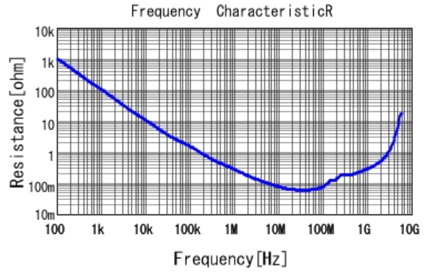
GRM188R71E103KA01 R DCOV, 25degC
