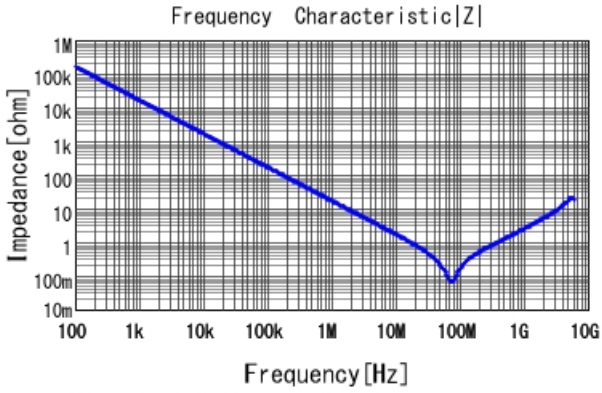
GRM188R71E103KA01 |Z| DCOV, 25degC
