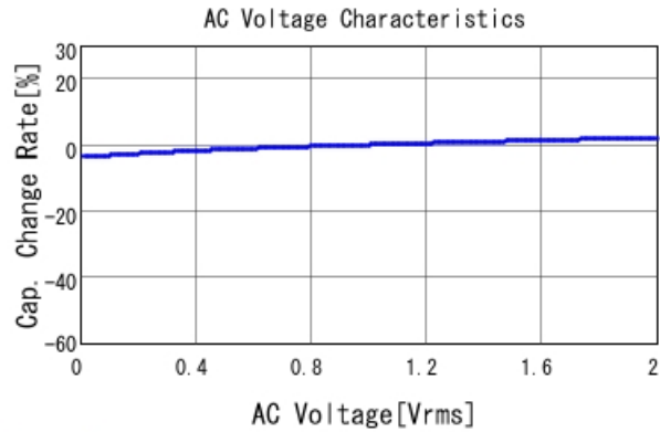
GRM188R71E103KA01 C-AC Voltage capchange, DCOV, 25
