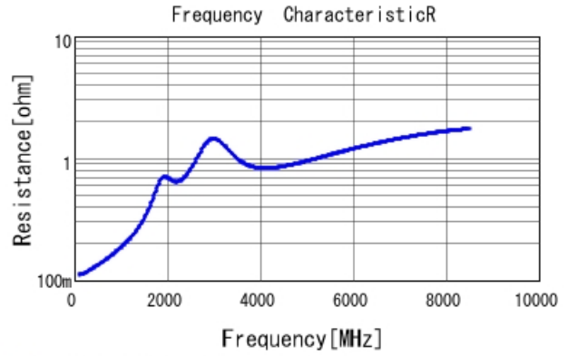
■ GRT1555C1H101JA02 R DC0V, 25degC
