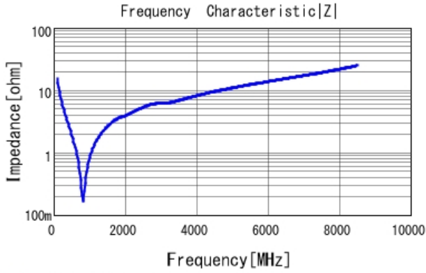
■ GRT1555C1H101JA02 |Z| DC0V, 25degC
