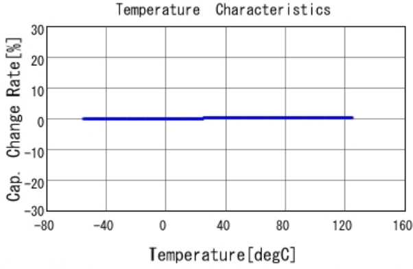
GRM1885C2A1R6BA01 C-Temp. capchange, DCOV, AC1Vrms
