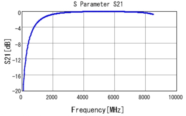
GRM1885C2A1R6BA01 S21 DCOV, 25degC
