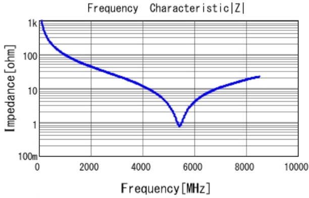
GRM1885C2A1R6BA01 |Z| DCOV, 25degC
