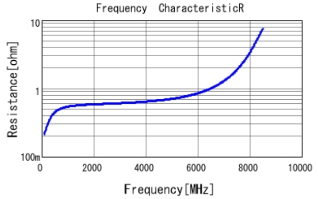
GRM1885C2A1R6BA01 R DCOV, 25degC
