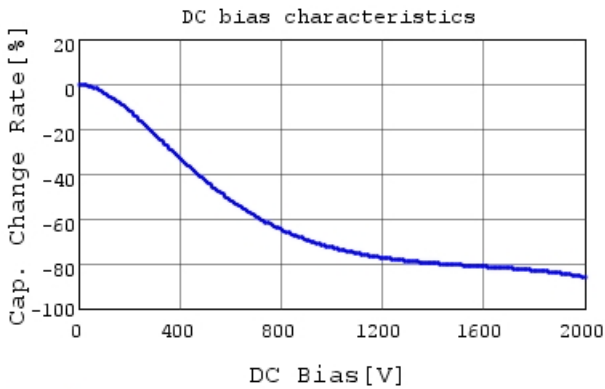
GR442QR73D152KW01 C-DC bias capchange, 25.0c
