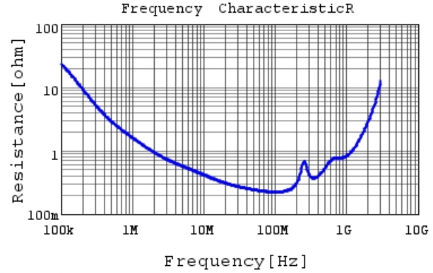
GR442QR73D152KW01 R DCOV, 25degC
