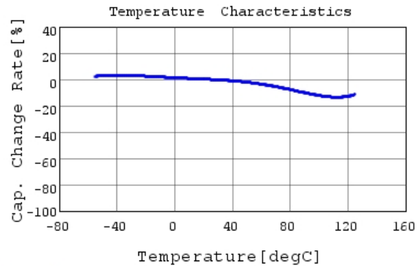
GR442QR73D152KW01 C-Temp. capchange, DCOV, 1
