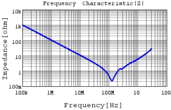
GR442QR73D152KW01 |Z| DCOV, 25degC
