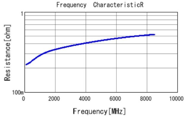
GRM0225C1E2R5CA03 R DCOV, 25degC
