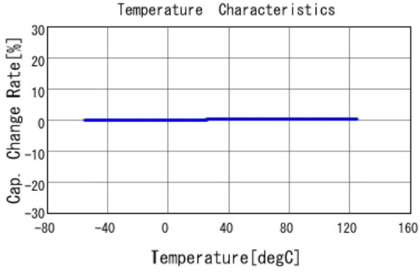
GRM0225C1E2R5CA03 C-Temp. capchange, DC0V, AC1Vrms
