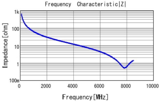
GRM0225C1E2R5CA03 |Z| DCOV, 25degC
