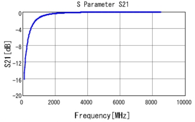
GRM0225C1E2R5CA03 S21 DC0V, 25degC
