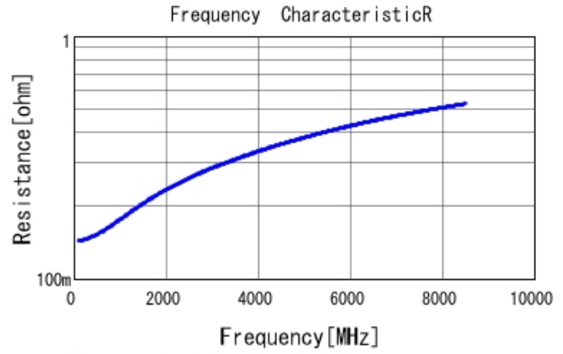
GRM0225C1E6R5WA03 R DCOV, 25degC
