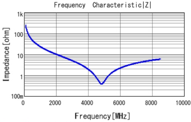
GRM0225C1E6R5WA03 |Z| DCOV, 25degC
