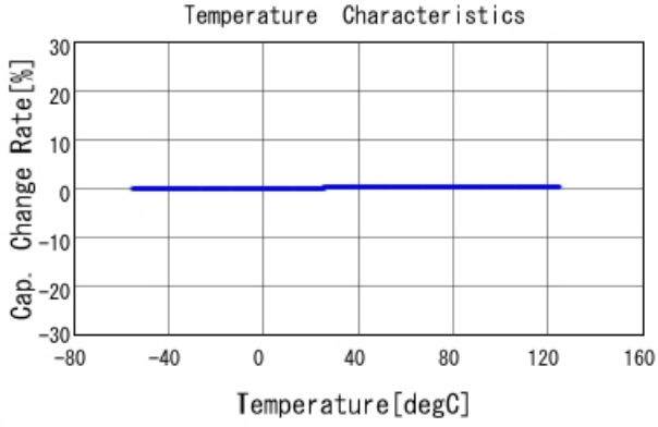
GRM0225C1E6R5WA03 C-Temp. capchange, DCOV, AC1Vrms
