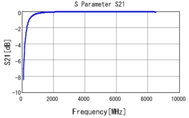
GRM0225C1E6R5WA03 S21 DCOV, 25degC
