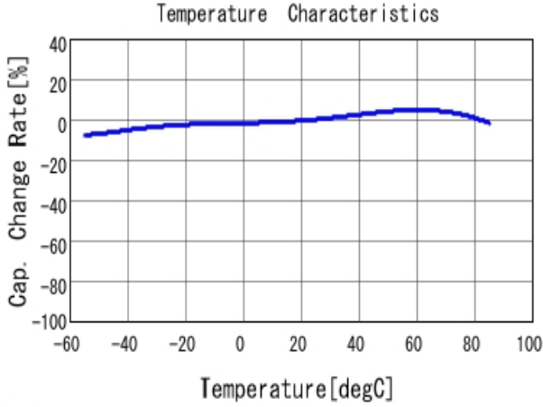
■ GRT31CR61E106KE01 C-Temp. capchange, DC0.0V, AC1.0V r m
