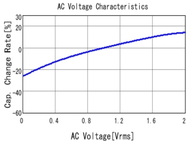
■ GRT31CR61E106KE01 C-AC Voltage capchange, DCOV, 25.0d
