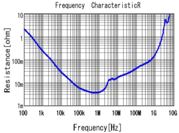
■ GRT31CR61E106KE01 R DCOV, 25degC
